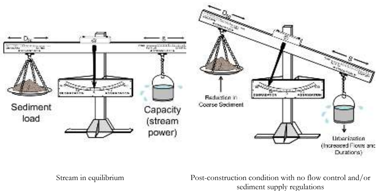
Figure H.4-1 Illustration of Lane's Relationship
