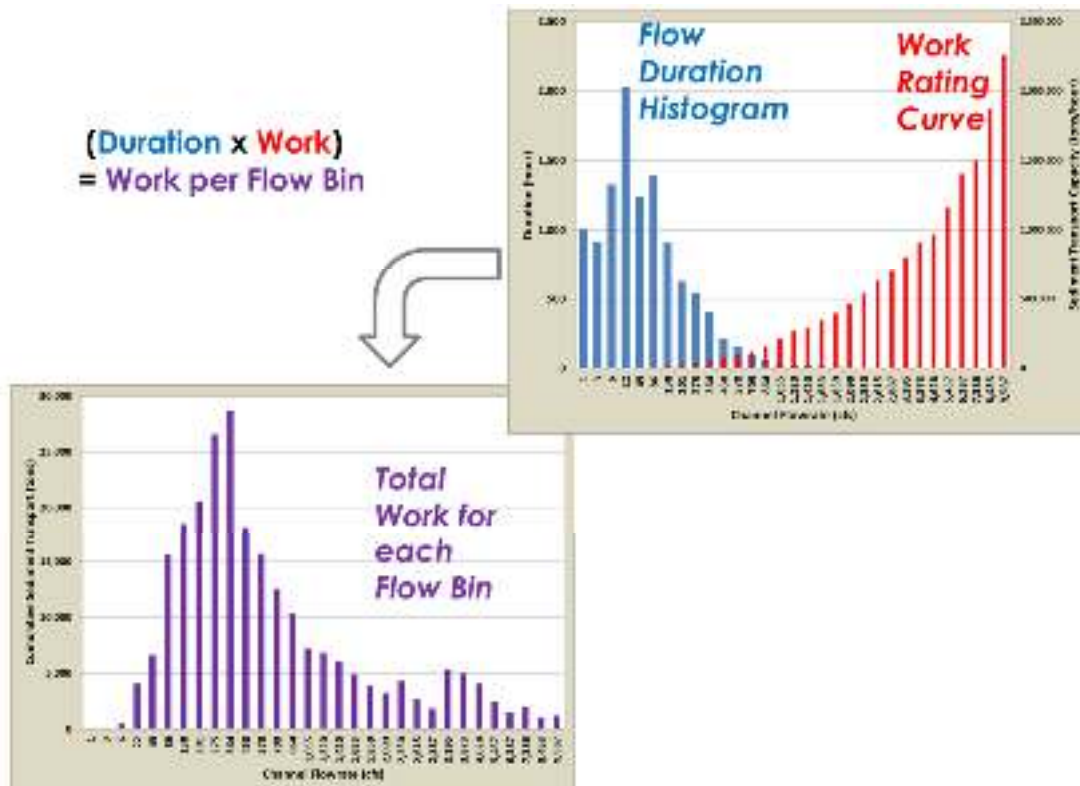
Figure H.8-5 Example Work Curve
