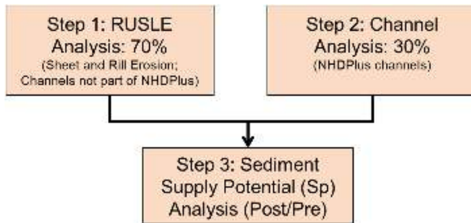
Figure H.8-8 Sediment Supply Potential Flow Chart
