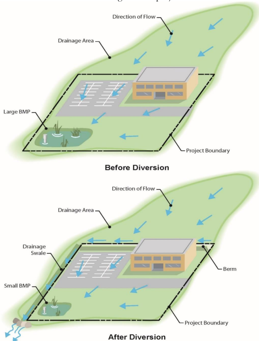
Figure 3-3 Tributary Area for BMP Sizing
