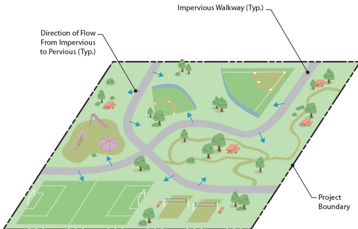
Figure 5-4: Self-retaining Site
