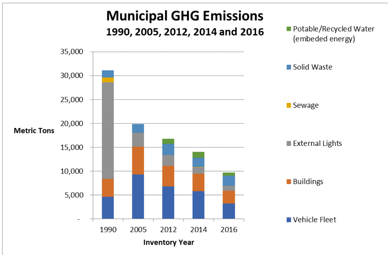
Figure 1: Total GHG emissions from municipal sources (by sector) in 1990, 2005, 2012, and 2014. Due to a lack of available data, emissions from the water sector are not included in the 1990 and 2005 inventories.
