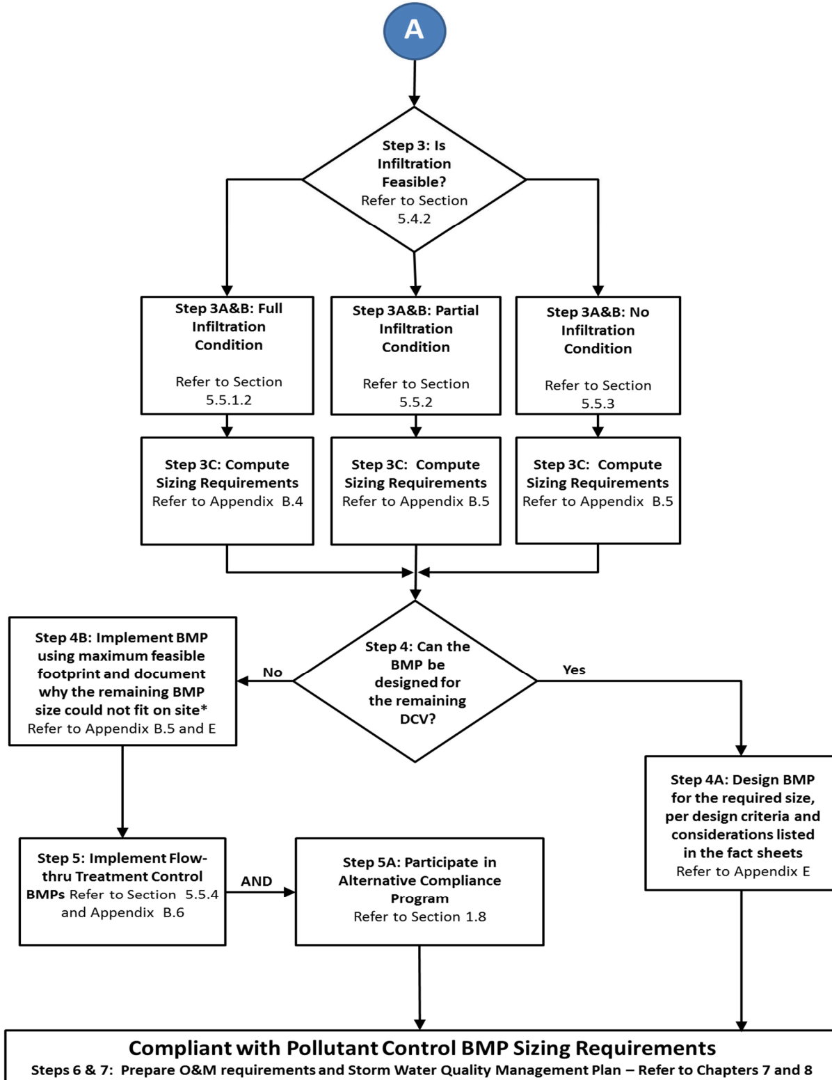
Figure 5-2: Storm Water Pollutant Control BMP Selection Flow Chart
