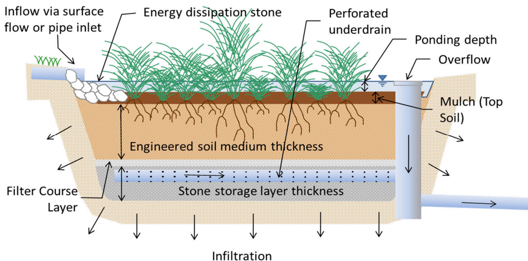
Figure 5-8: Schematic of a Typical Biofiltration with Partial Retention BMP
