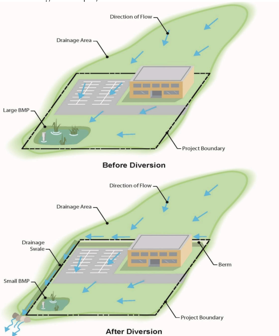
Figure 3-3 Tributary Area for BMP Sizing
