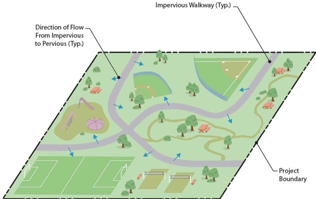
Figure 5-4: Self-retaining Site
