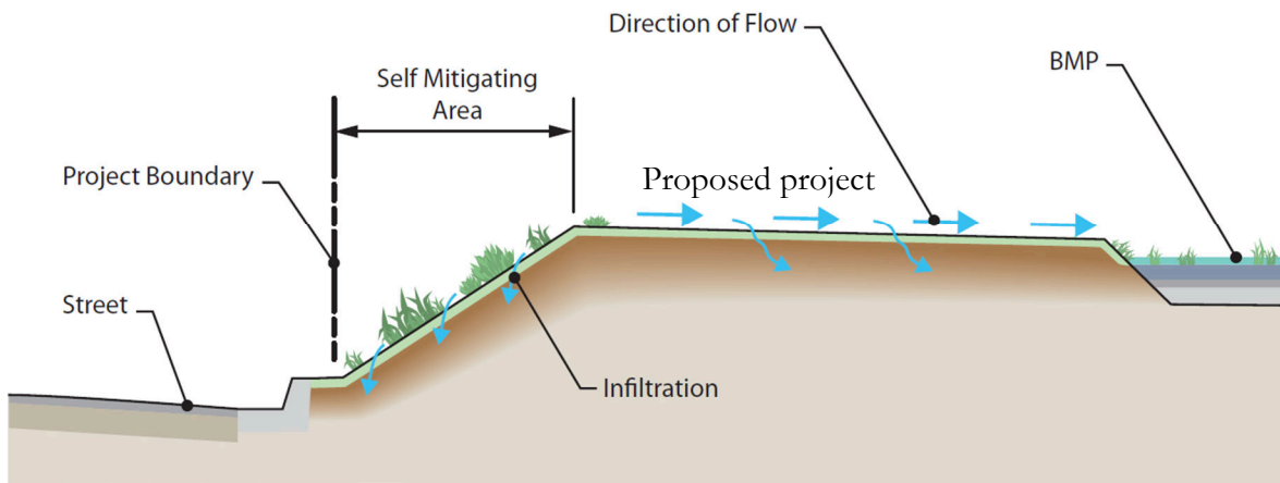
Figure 5-3: Self Mitigating Area
