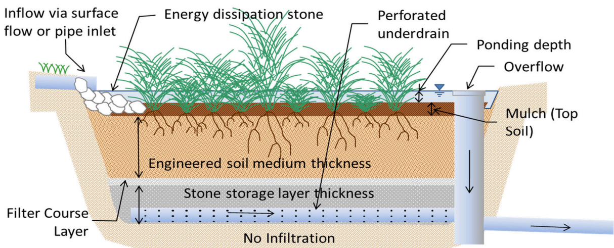
Figure 5-9: Schematic of a Typical Biofiltration Basin
