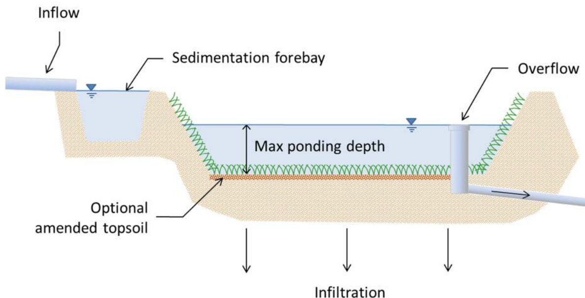
Figure 5-7: Schematic of a Typical Infiltration Basin
