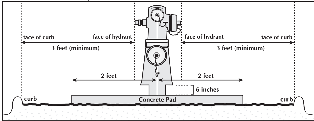
SIDE VIEW
