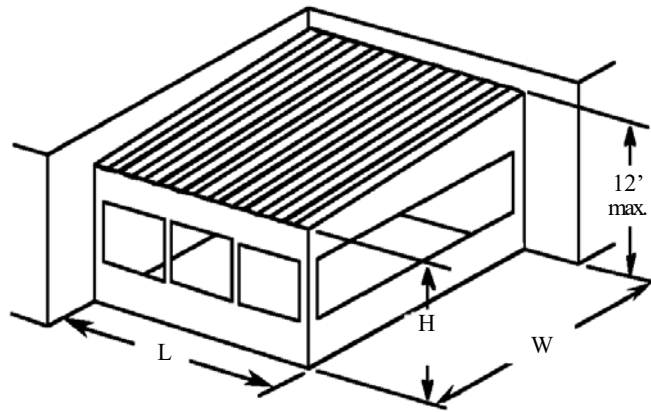
FIGURE 2 / Patio cover with two adjacent sides open
