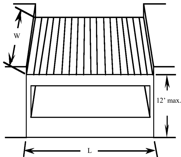
FIGURE 4 / Patio cover with one side open
